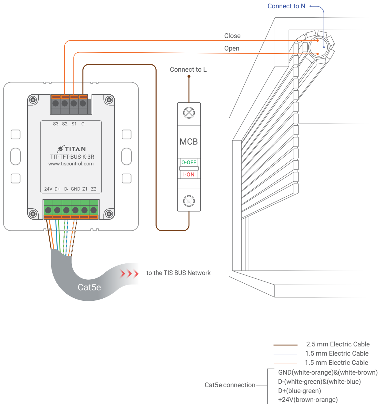
▲ Figure 4: TIT-TFT-BUS-K-3R & Motors Connection Diagram
