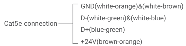
▲ Figure 7: TIT-4G-BUS-S-3R Module's Bus Connection Color Coding
