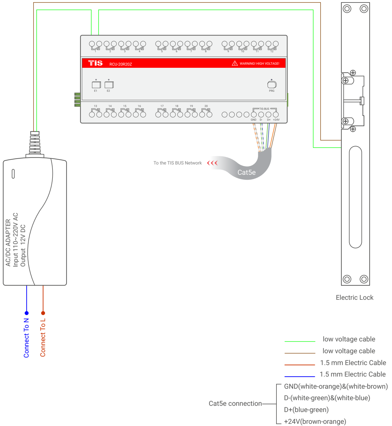
▲ Figure 4: Electric Lock Connection Diagram
