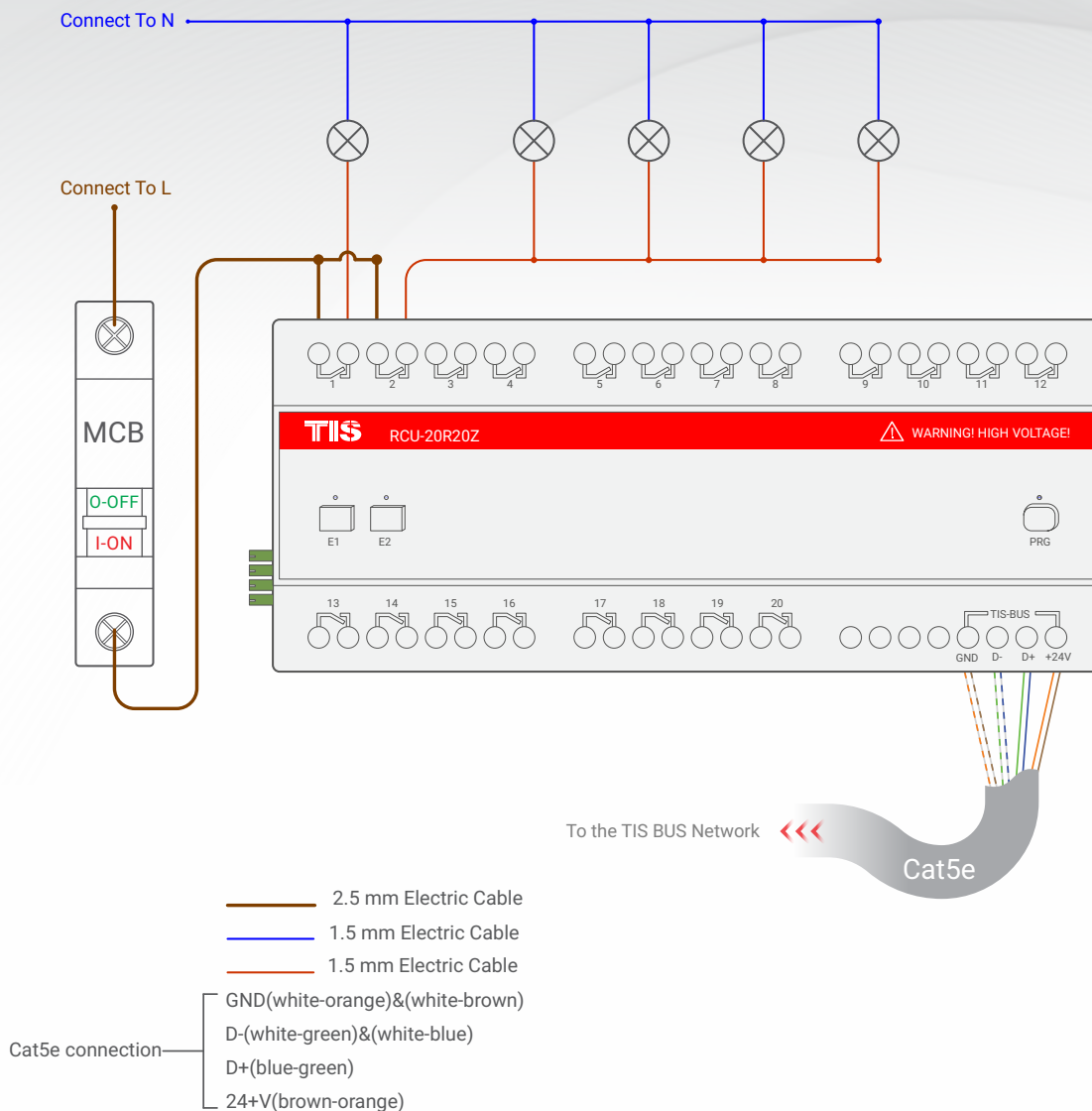
▲ Figure 1: Lights Connection Diagram
