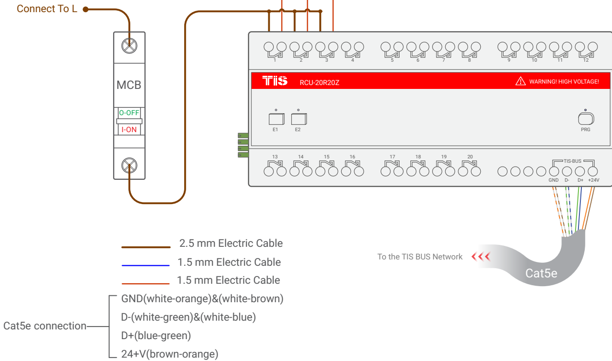
▲ Figure 2: FCU Connection Diagram
